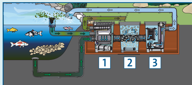
Module filters ProfiClear Premium gravity fed system
