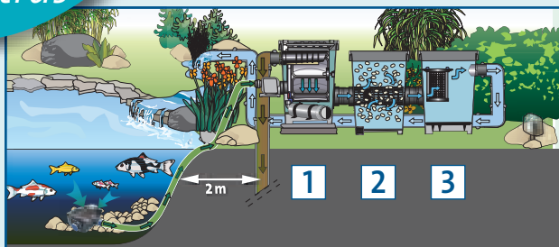
Module filters ProfiClear Premium pump fed system
